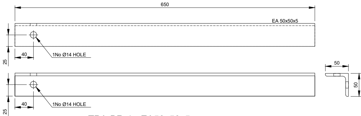
TPA-BR-1 - EA50x50x5 Scale 1:5
