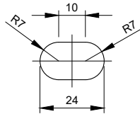
SLOTTED HOLE DETAIL Scale 1:2
