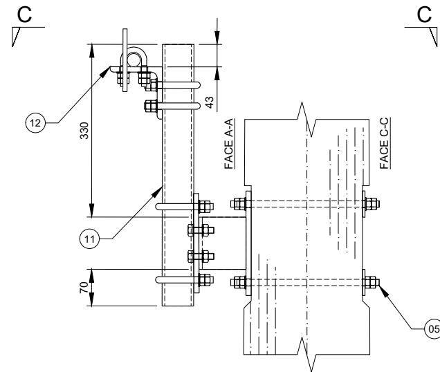
DETAIL H - Rx ANTENNA MOUNT Scale 1:10
