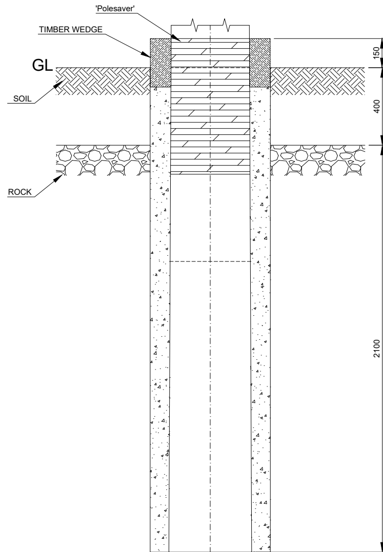
POROPOSED INSTALLATION ELEVATION Scale 1:20
