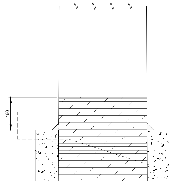
WATER PROOFING Scale 1:10
