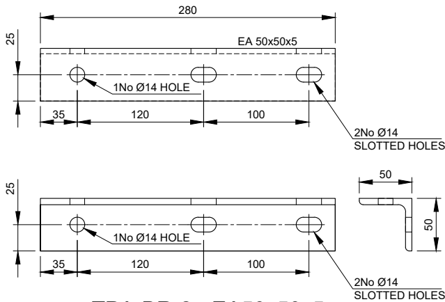
TPA-BR-2 - EA50x50x5 Scale 1:5
