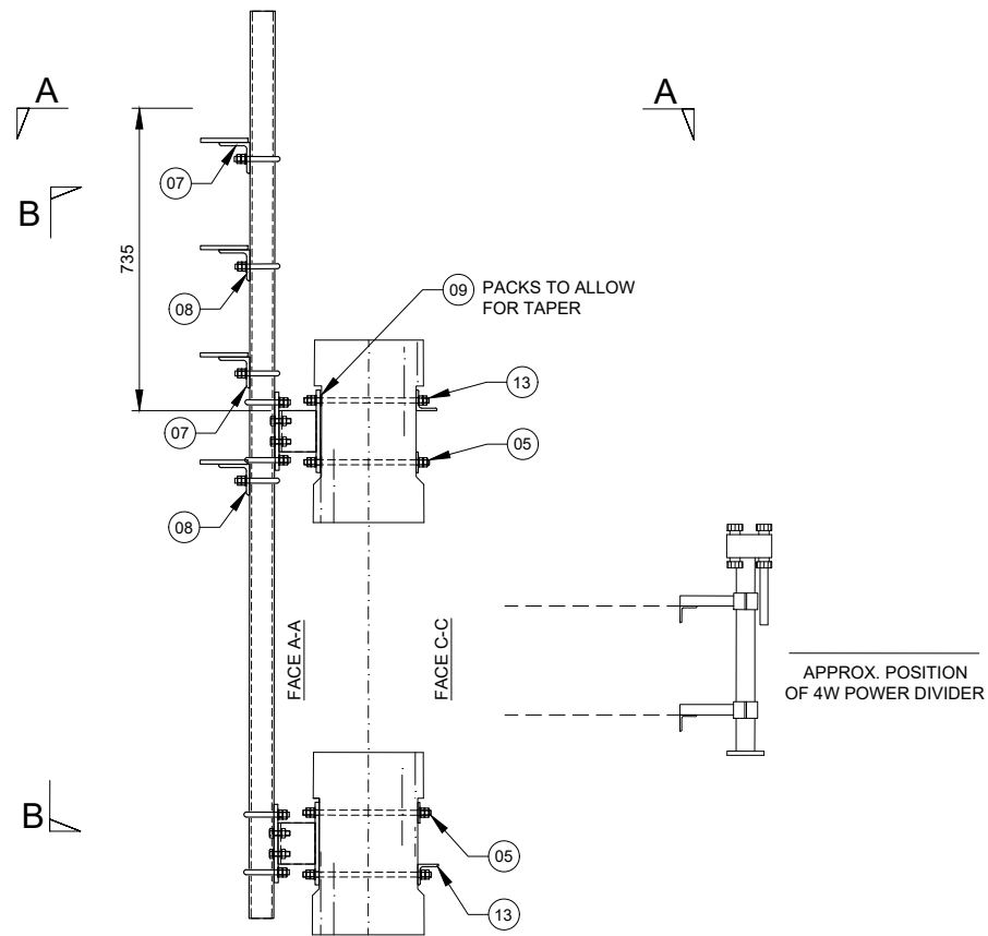
DETAIL G - Tx ANTENNA MOUNT Scale 1:20
