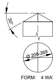
DETAIL A - TIMBER POLE TOP Scale 1:20
