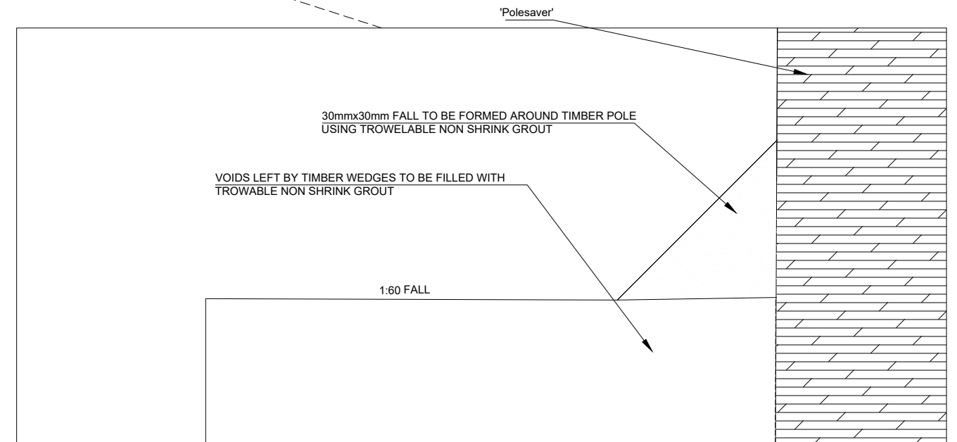
ENLARGED DETAIL Scale 1:1
