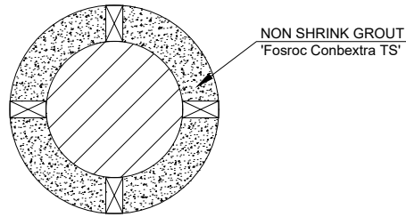
POROPOSED INSTALLATION PLAN VIEW Scale 1:20
