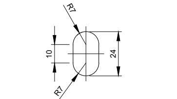
SLOTTED HOLE DETAIL Scale 1:2
